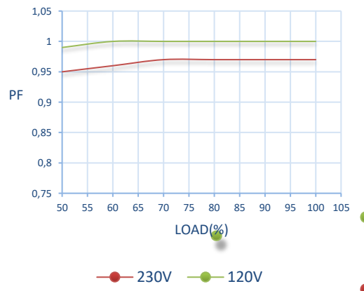
PF CURVE
