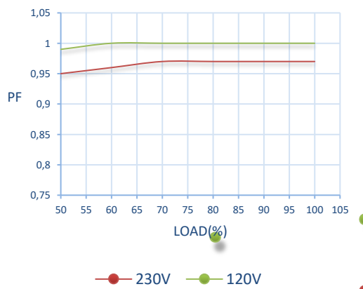
PF CURVE
