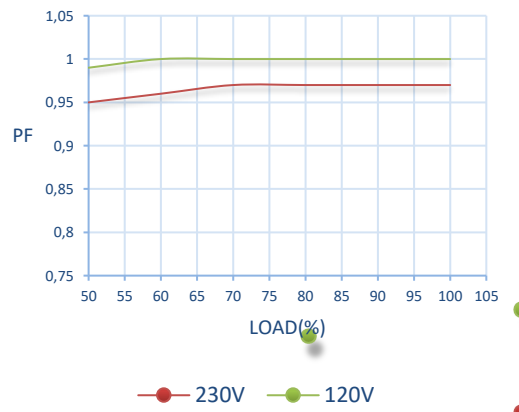
PF CURVE
