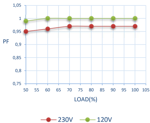
PF CURVE
